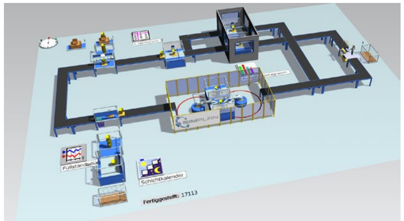
Example model of an assembly plant (SimPlan)
