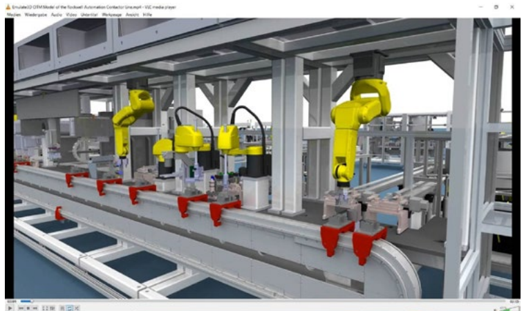
Emulate3D Model of assembly line (SimPlan)
