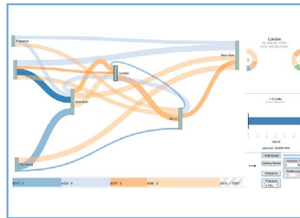
Sankey
